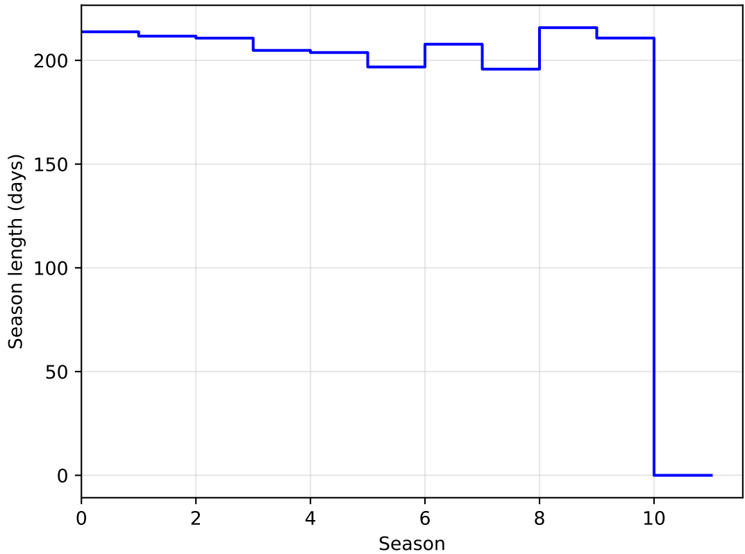
weather_cloudso30v3.5_10yrs DD:ECDFS all bands: SeasonLength
