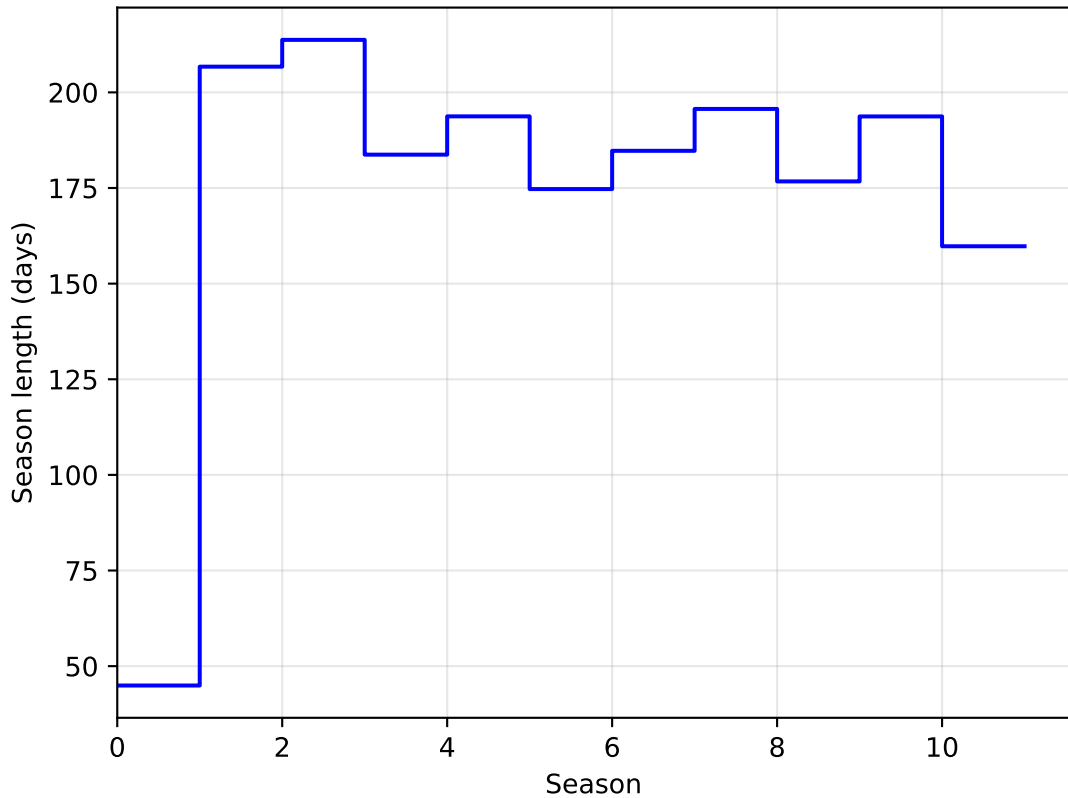
weather_cloudso30v3.5_10yrs DD: COSMOS all bands: SeasonLength
