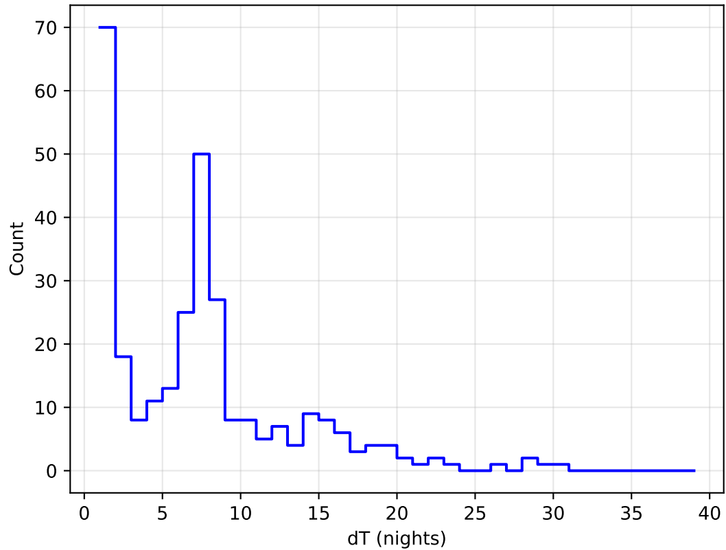
weather_cloudso30v3.5_10yrs all bands: DD:XMM_LSS Delta Nights Histogram
