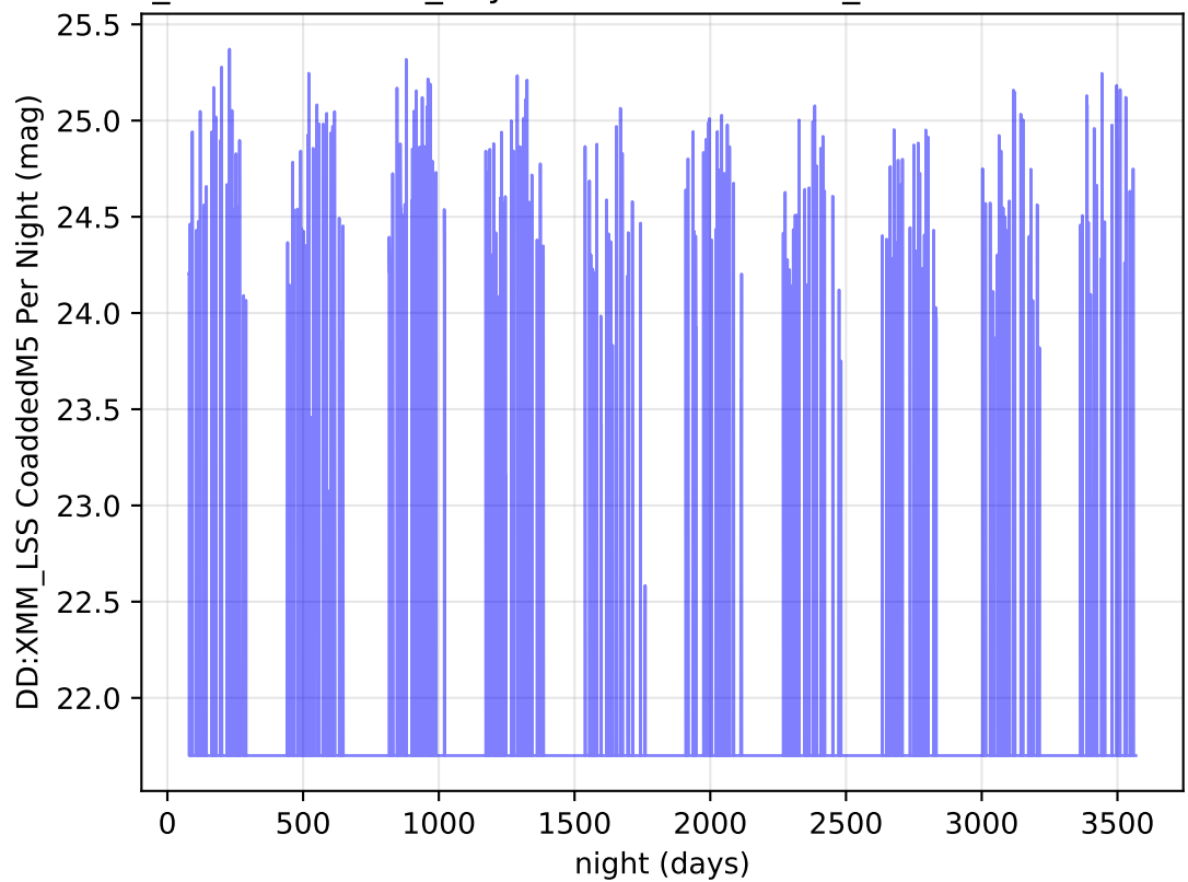
weather_cloudso30v3.5_10yrs z band: DD:XMM_LSS CoaddedM5 Per Night
