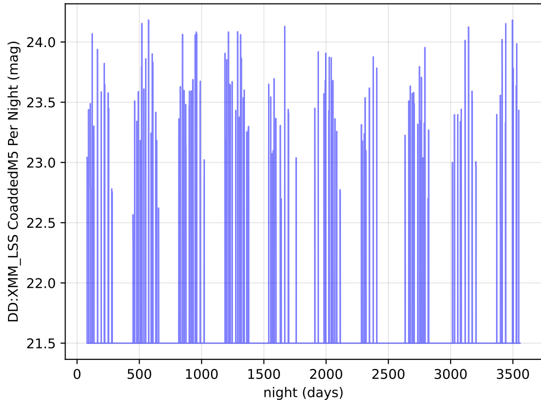
weather_cloudso30v3.5_10yrs y band: DD:XMM_LSS CoaddedM5 Per Night
