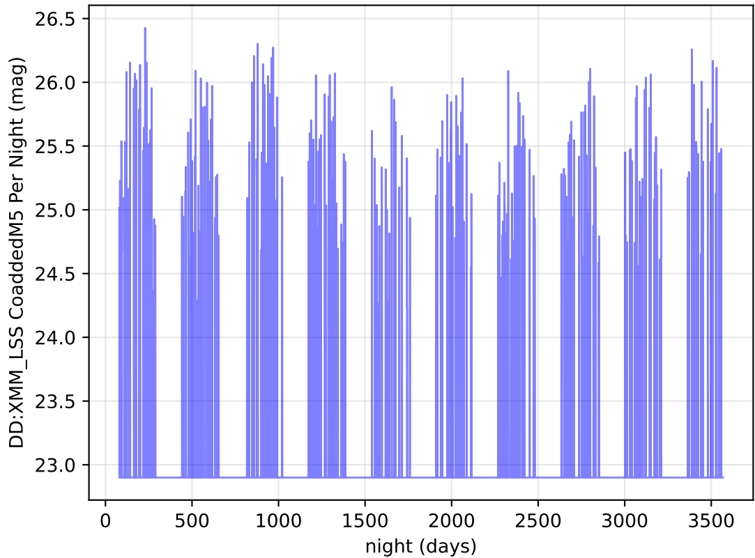
weather_cloudso30v3.5_10yrs r band: DD:XMM_LSS CoaddedM5 Per Night
