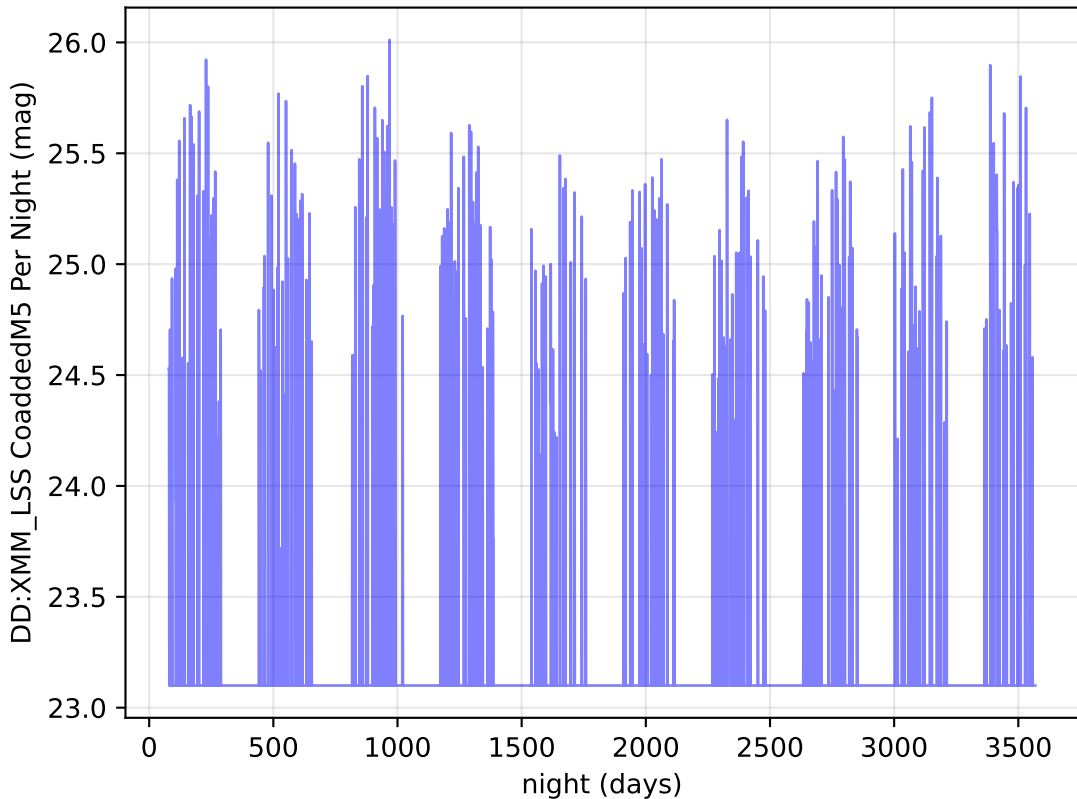
weather_cloudso30v3.5_10yrs i band: DD:XMM_LSS CoaddedM5 Per Night
