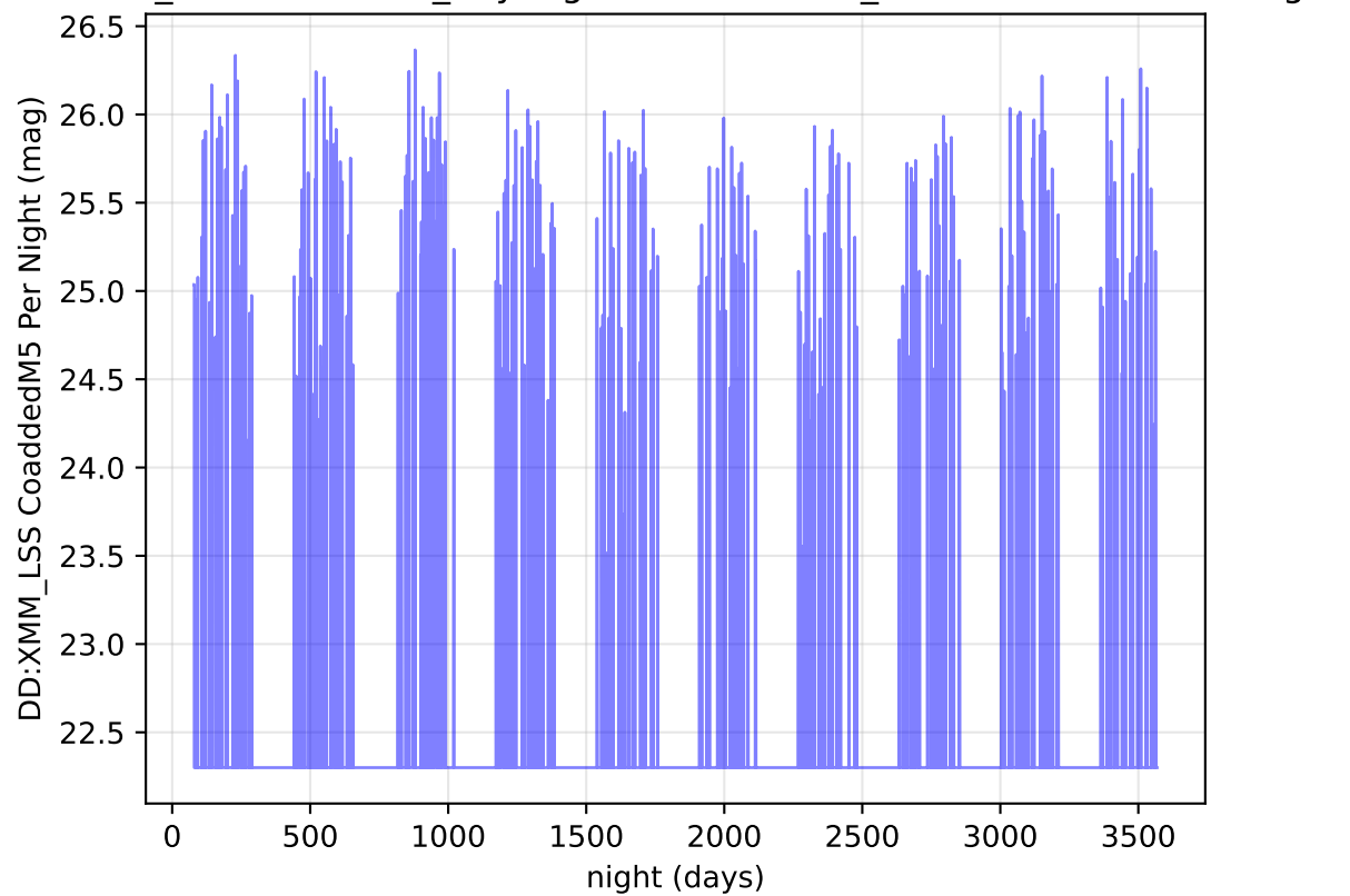
weather_cloudso30v3.5_10yrs g band: DD:XMM_LSS CoaddedM5 Per Night
