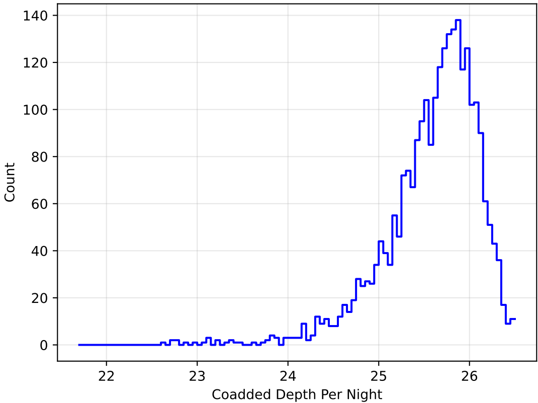
weather_cloudso30v3.5_10yrs z band: DD:WFD CoaddM5PerNight
