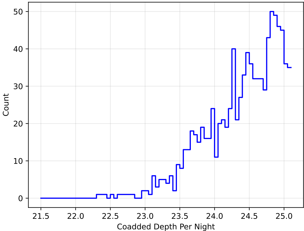
weather_cloudso30v3.5_10yrs y band: DD:WFD CoaddM5PerNight
