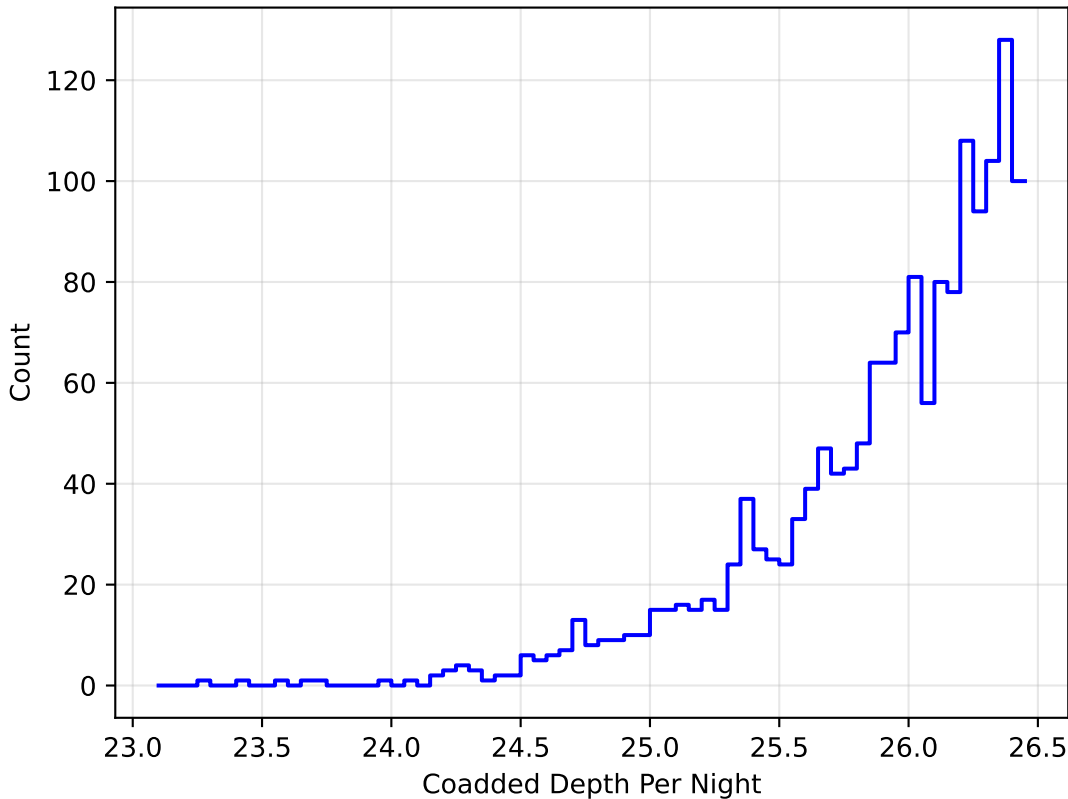
weather_cloudso30v3.5_10yrs i band: DD:WFD CoaddM5PerNight
