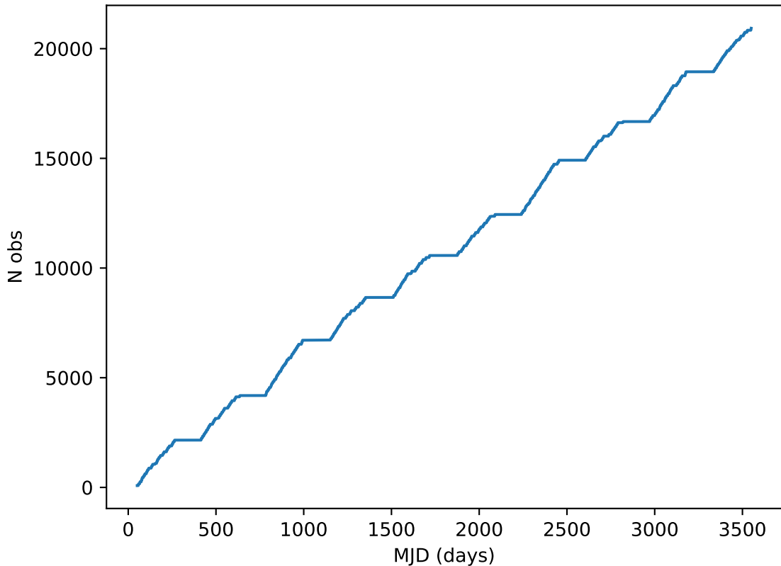
weather_cloudso30v3.5_10yrs all bands: DD:ELAISS1 Cumulative NVisits
