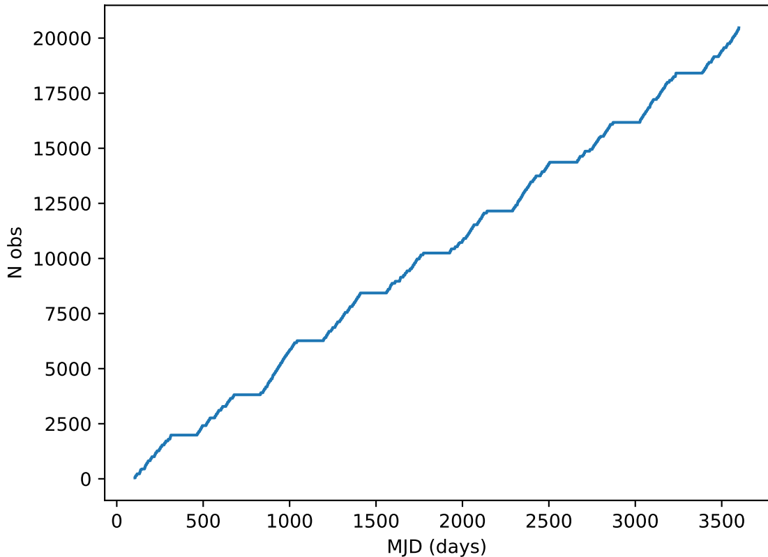
weather_cloudso30v3.5_10yrs all bands: DD:EDFS Cumulative NVisits
