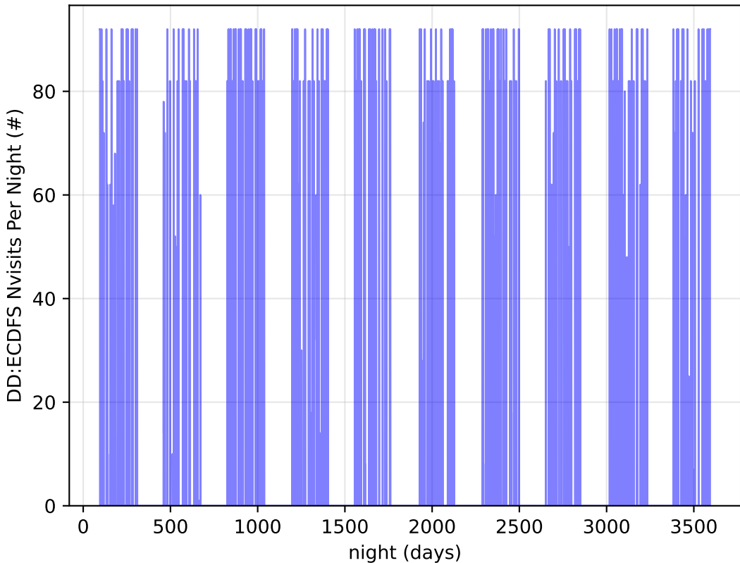
weather_cloudso30v3.5_10yrs all bands: DD:ECDFS Nvisits Per Night
