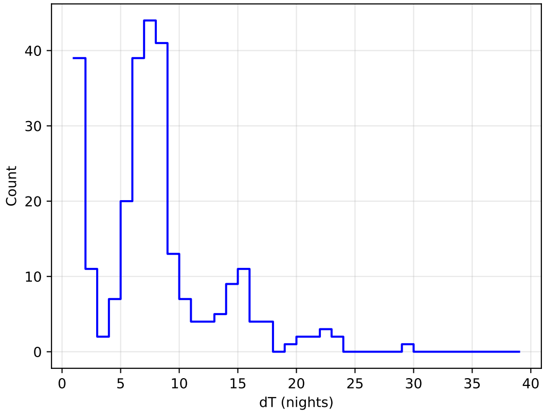
weather_cloudso30v3.5_10yrs all bands: DD:ECDFS Delta Nights Histogram
