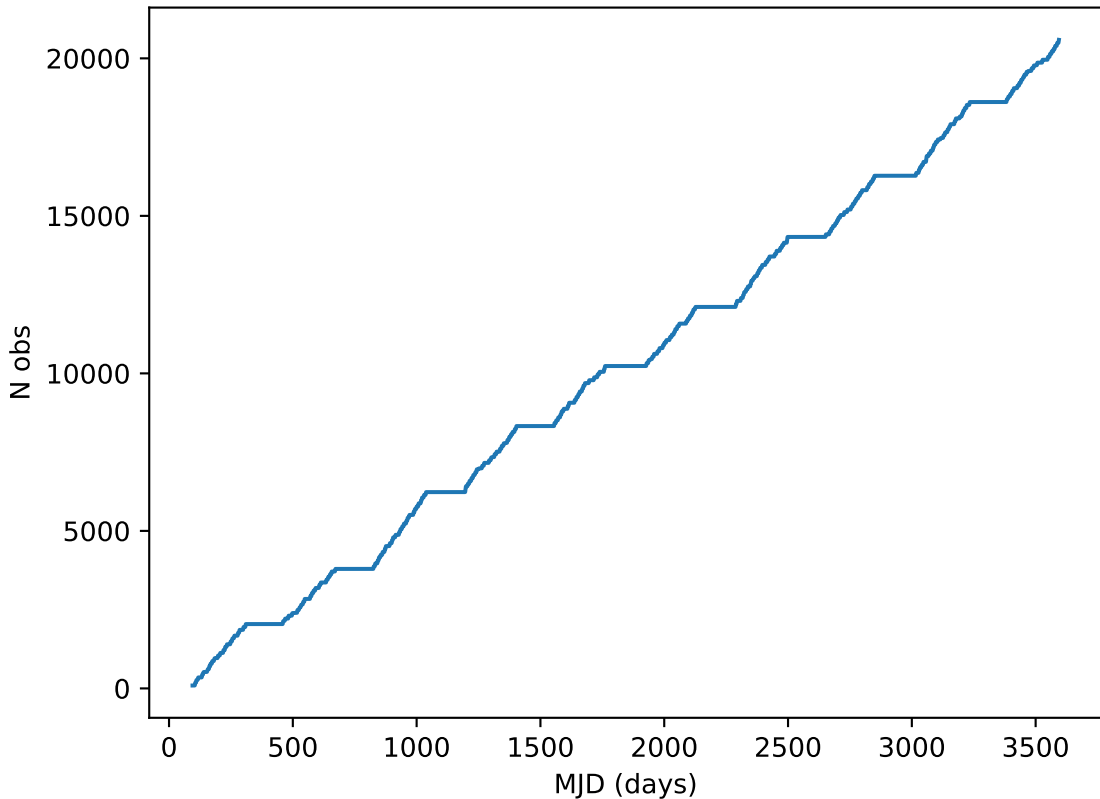
weather_cloudso30v3.5_10yrs all bands: DD:ECDFS Cumulative NVisits
