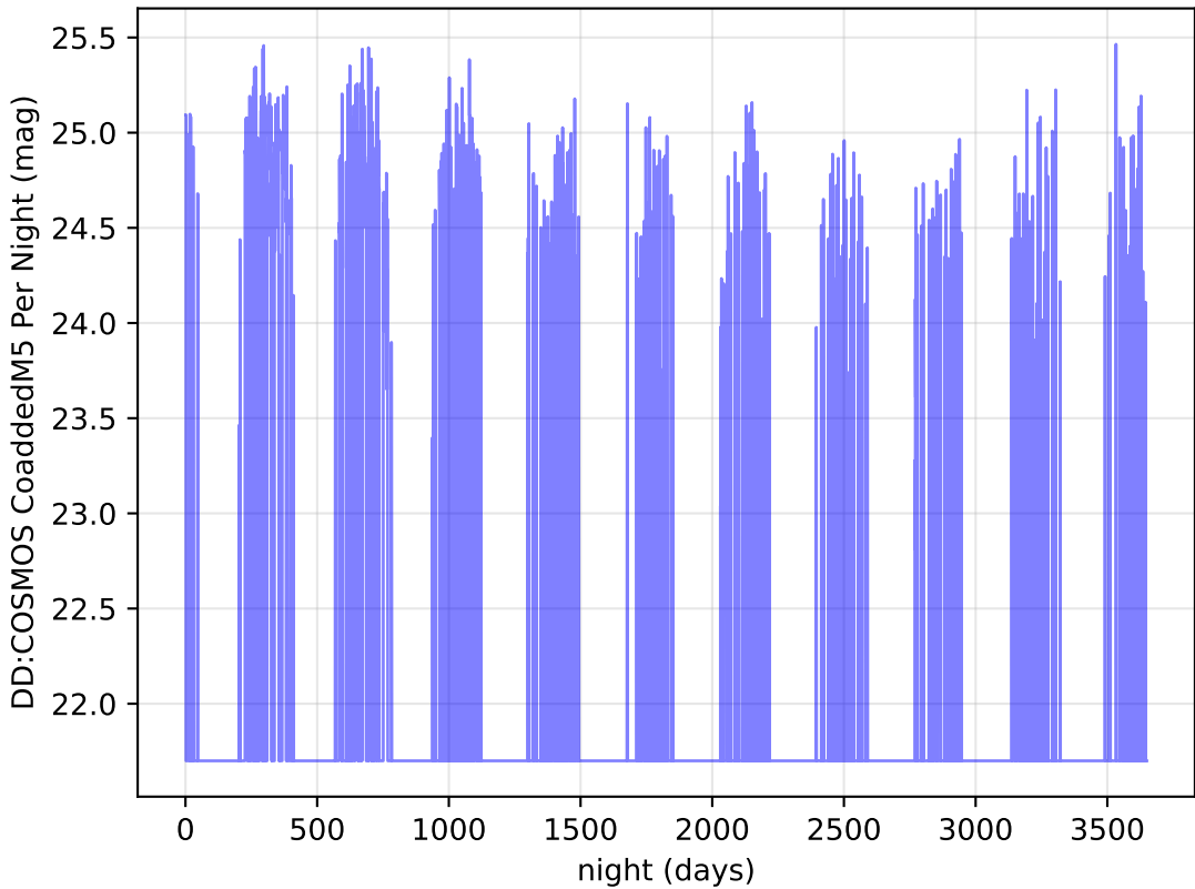
weather_cloudso30v3.5_10yrs z band: DD:COSMOS CoaddedM5 Per Night
