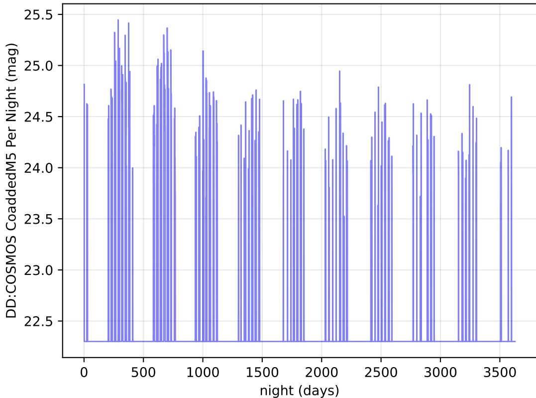
weather_cloudso30v3.5_10yrs u band: DD:COSMOS CoaddedM5 Per Night
