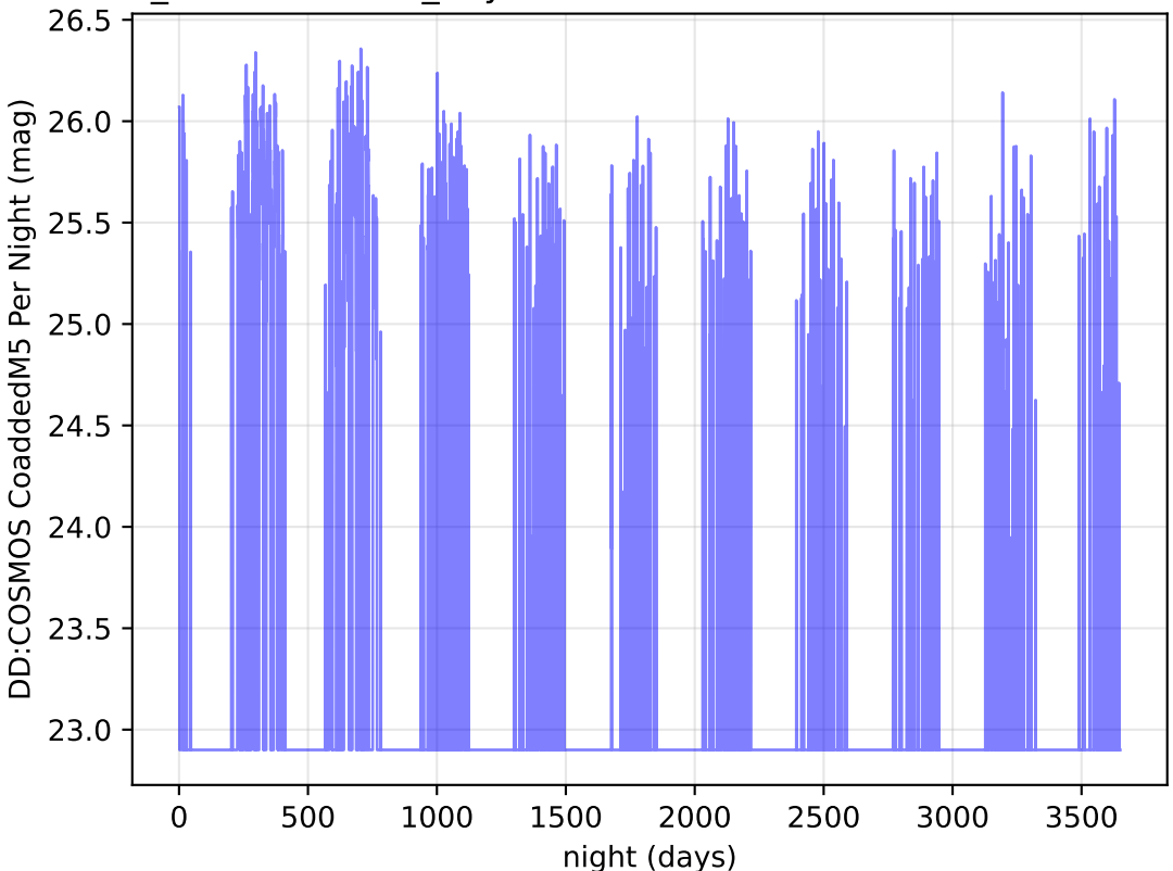
weather_cloudso30v3.5_10yrs r band: DD:COSMOS CoaddedM5 Per Night
