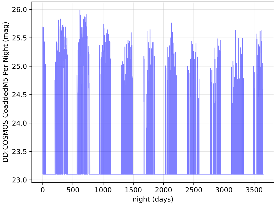
weather_cloudso30v3.5_10yrs i band: DD:COSMOS CoaddedM5 Per Night
