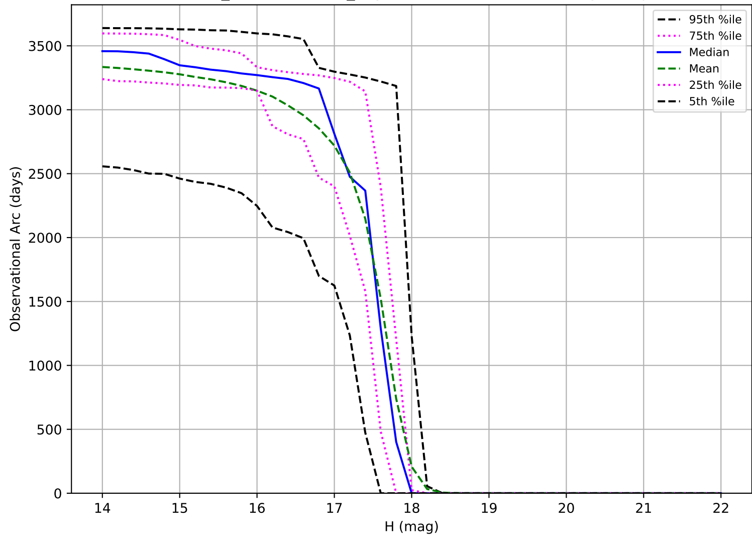
weather_cloudso30v3.4_10yrs: Observational Arc Length Trojan
