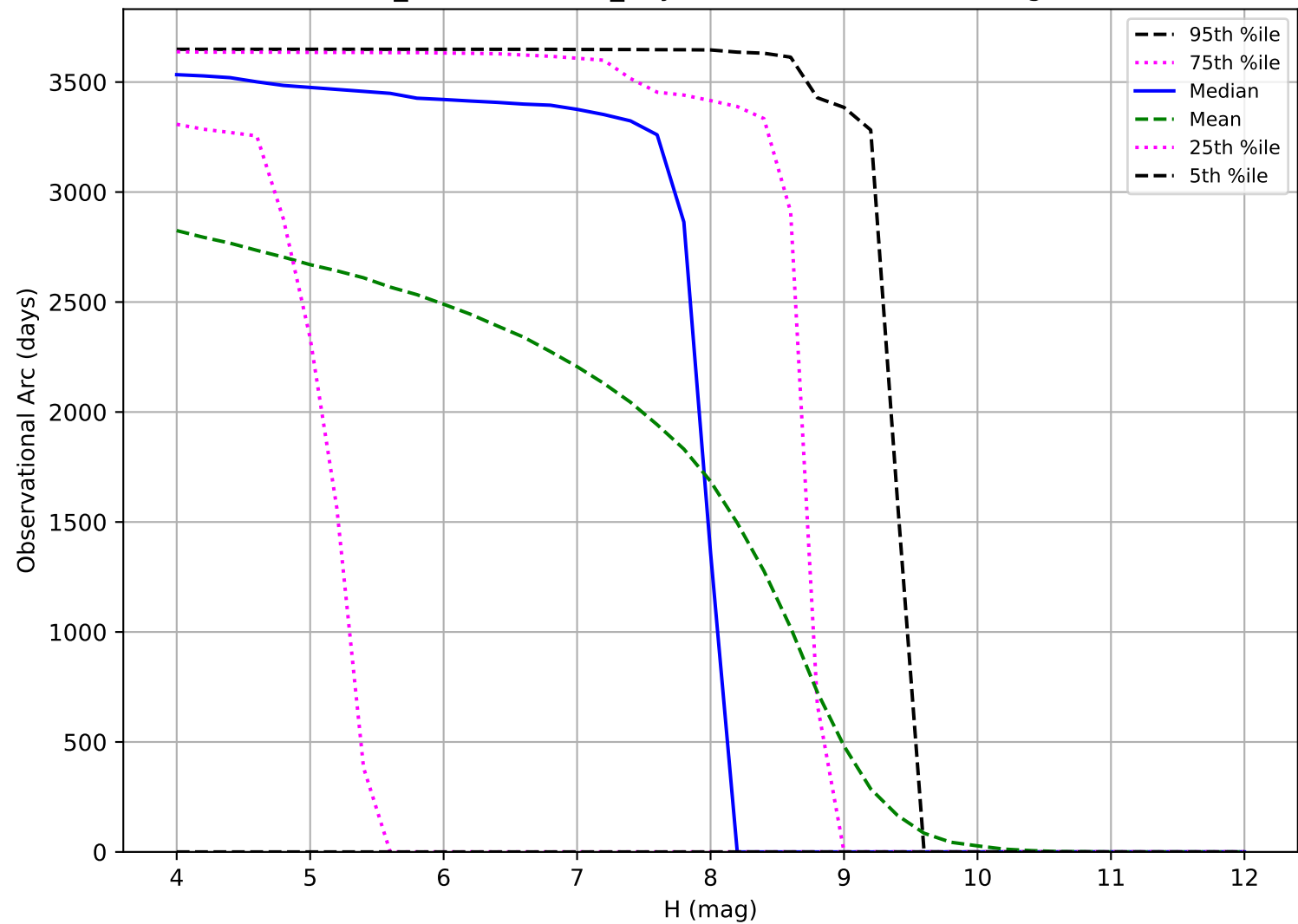
weather_cloudso30v3.4_10yrs: Observational Arc Length TNO
