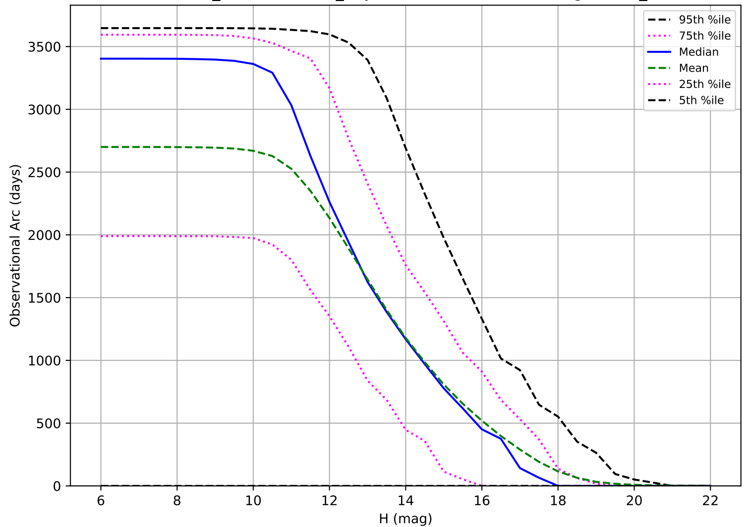
weather_cloudso30v3.4_10yrs: Observational Arc Length OCC_r5
