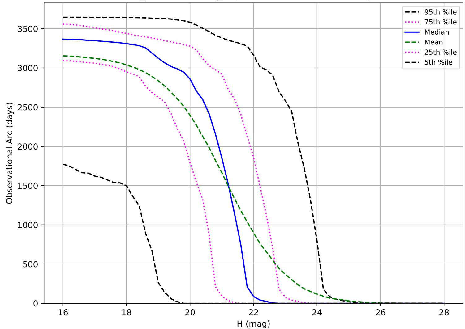
weather_cloudso30v3.4_10yrs: Observational Arc Length NEO
