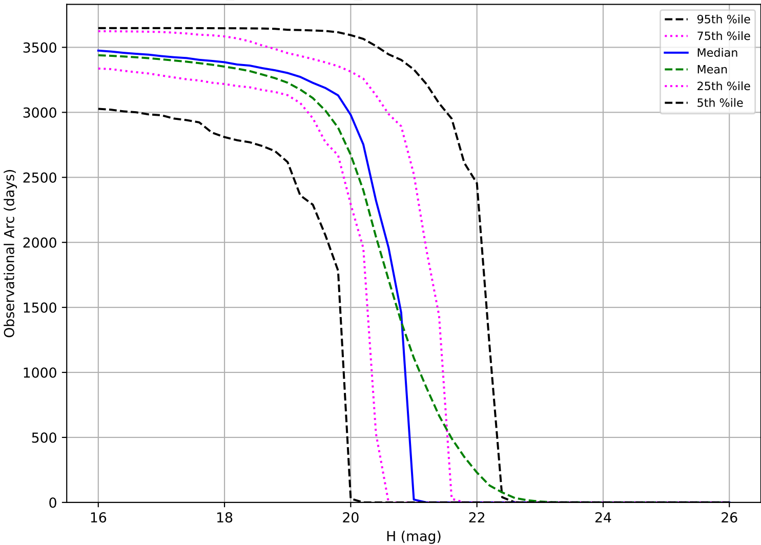
weather_cloudso30v3.4_10yrs: Observational Arc Length MBA
