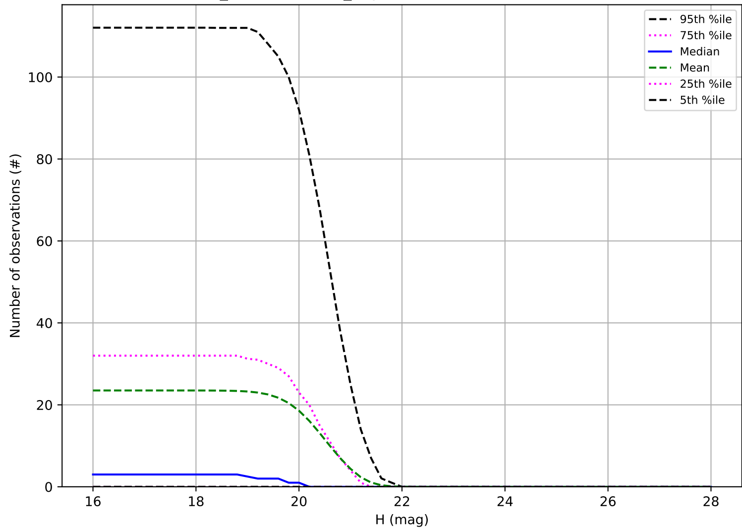
weather_cloudso30v3.4_10yrs: Number of observations Vatira
