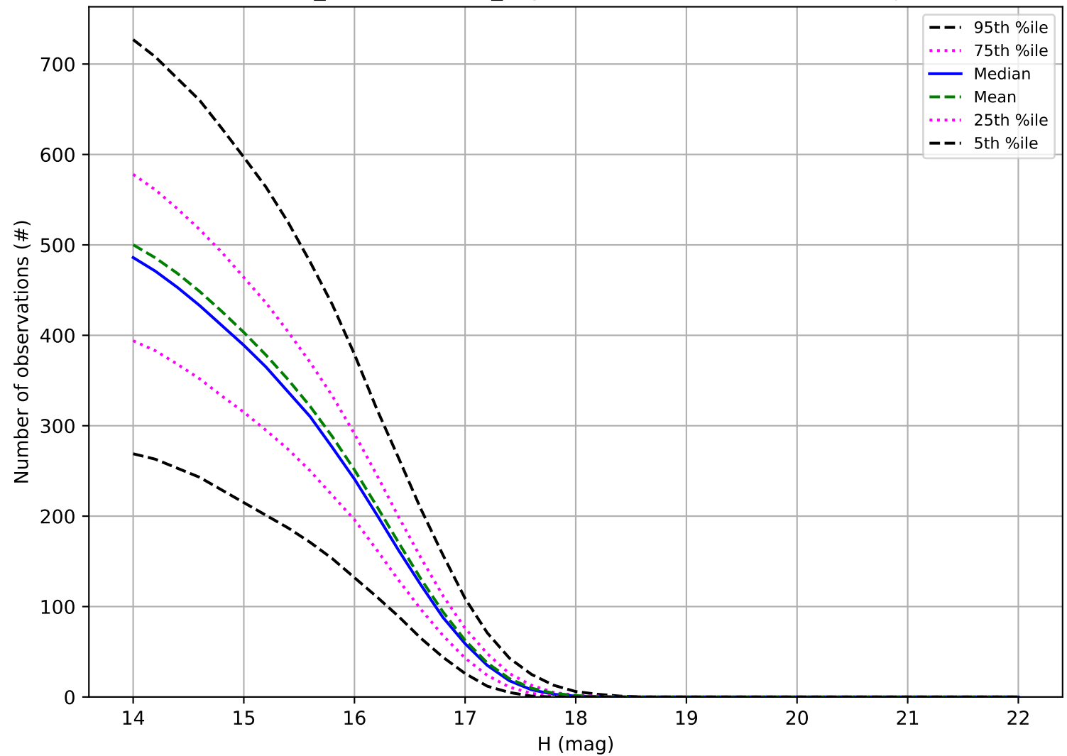
weather_cloudso30v3.4_10yrs: Number of observations Trojan
