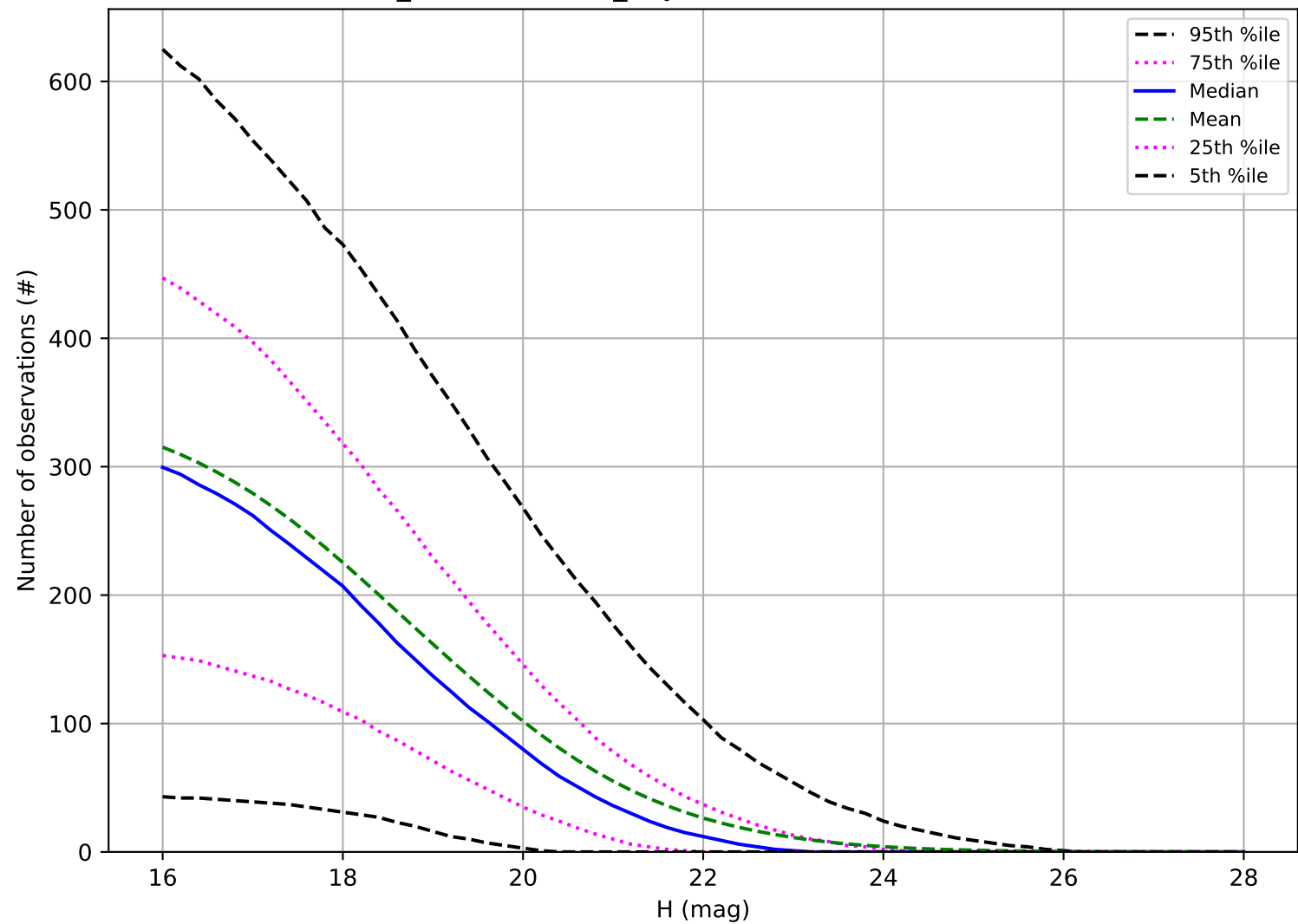
weather_cloudso30v3.4_10yrs: Number of observations PHA
