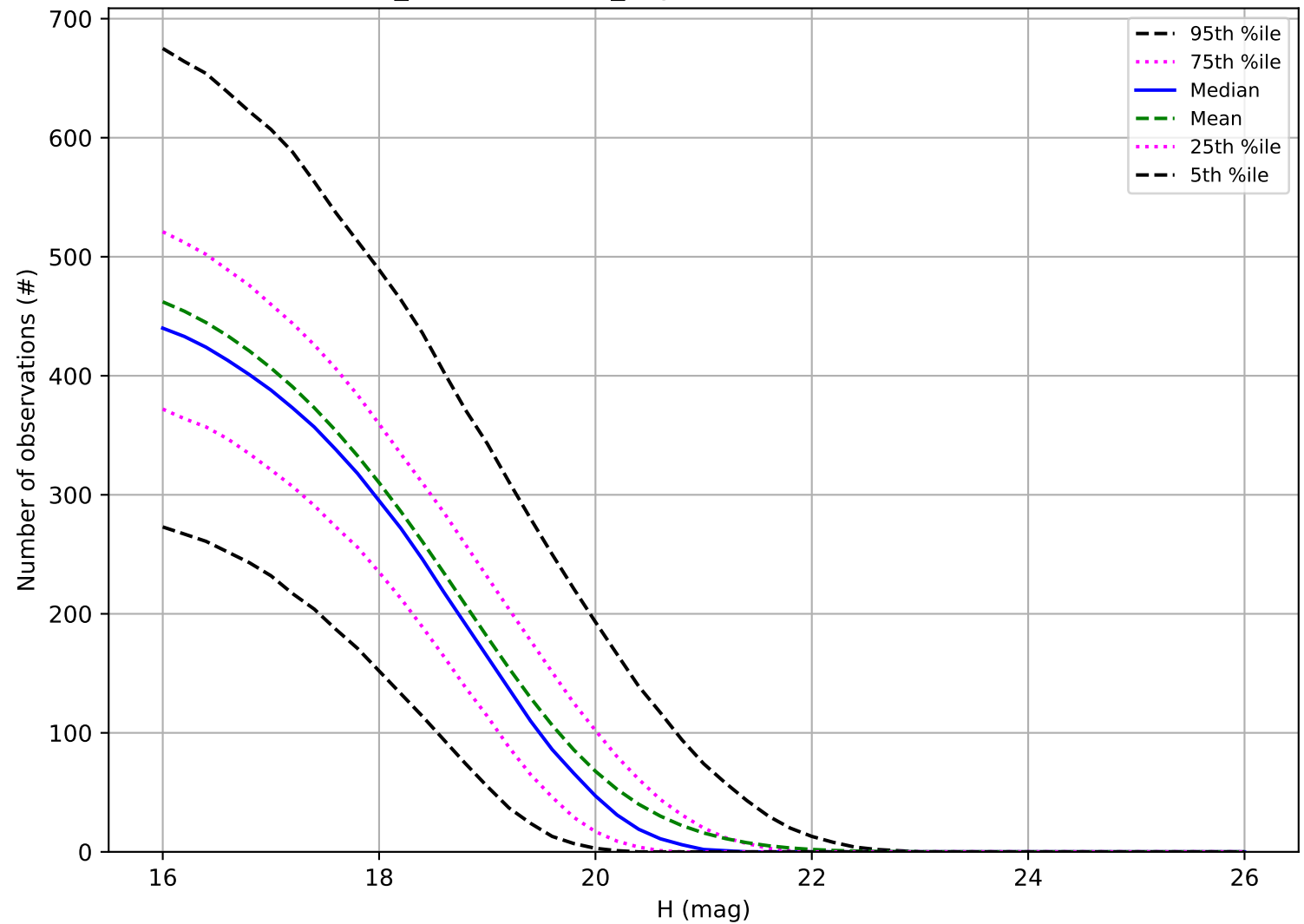
weather_cloudso30v3.4_10yrs: Number of observations MBA
