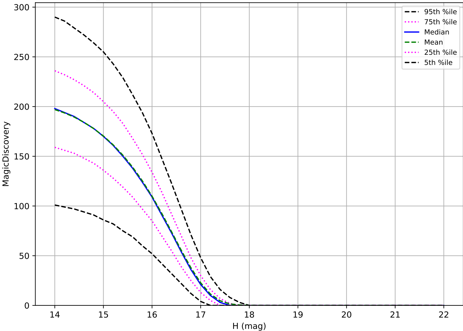
weather_cloudso30v3.4_10yrs: Trojan 6 detections in 60 nights detection loss
