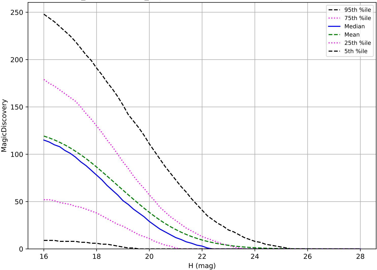
weather_cloudso30v3.4_10yrs: PHA 6 detections in 60 nights detection loss
