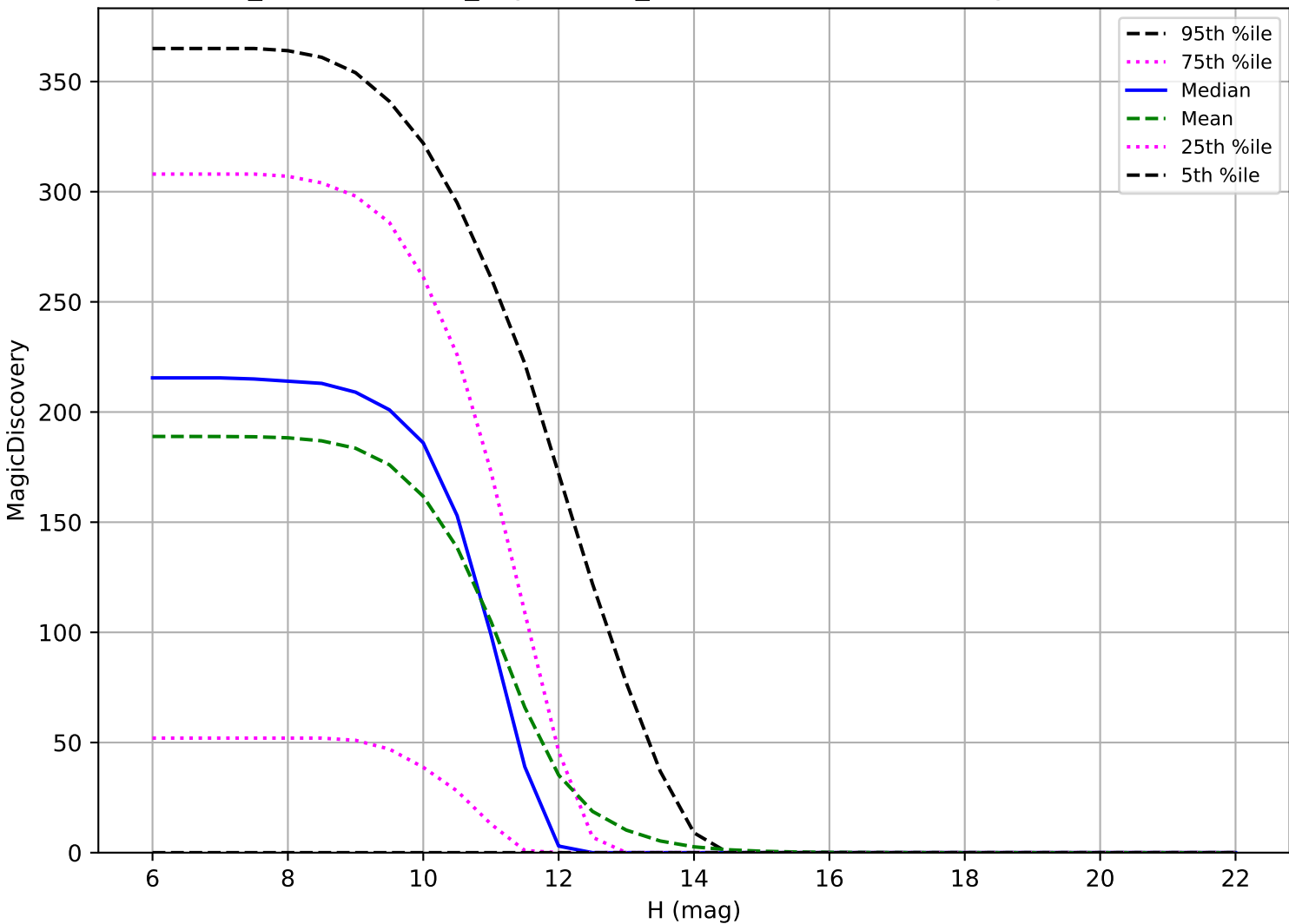
weather_cloudso30v3.4_10yrs: OCC_r20 6 detections in 60 nights detection loss
