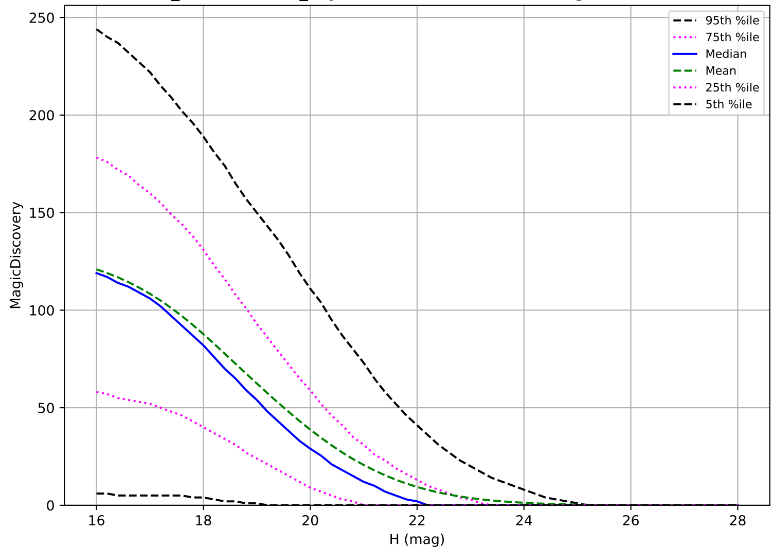
weather_cloudso30v3.4_10yrs: NEO 6 detections in 60 nights detection loss
