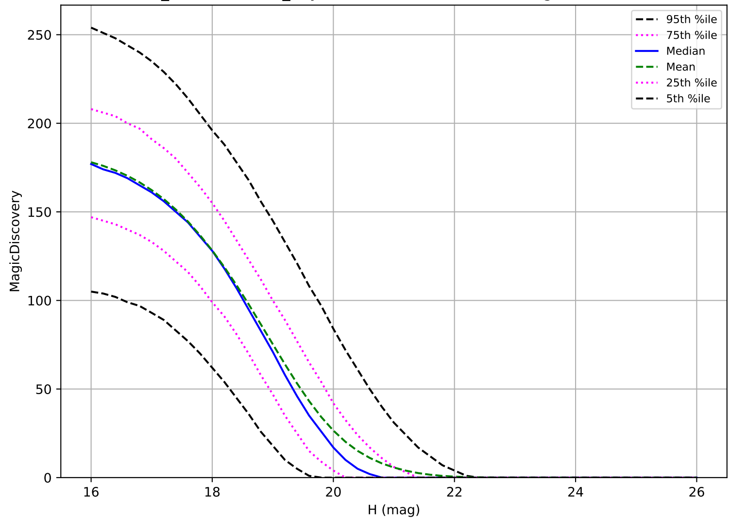
weather_cloudso30v3.4_10yrs: MBA 6 detections in 60 nights detection loss
