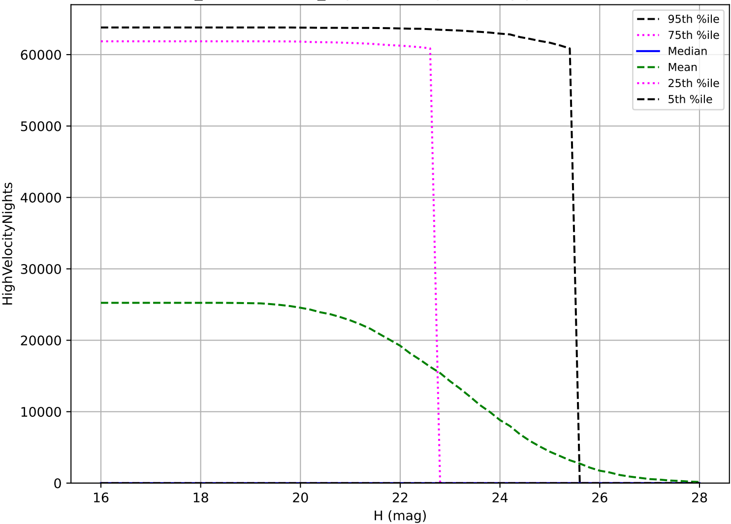
weather_cloudso30v3.4_10yrs: PHA High velocity pair detection loss
