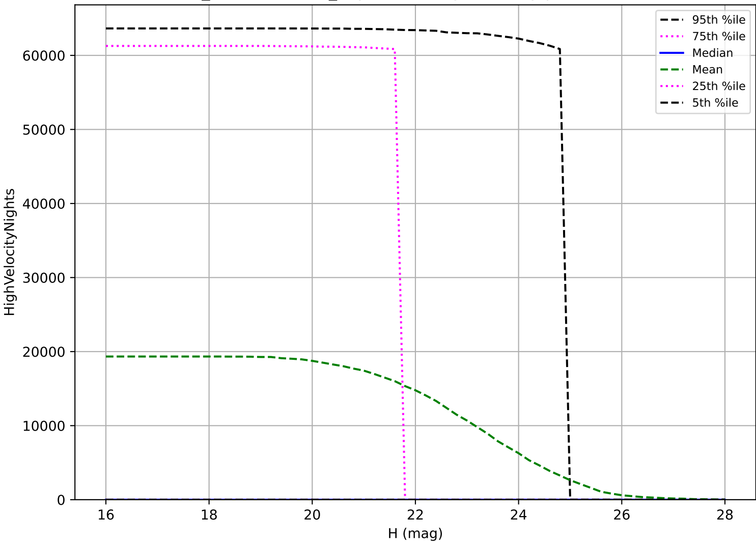
weather_cloudso30v3.4_10yrs: NEO High velocity pair detection loss
