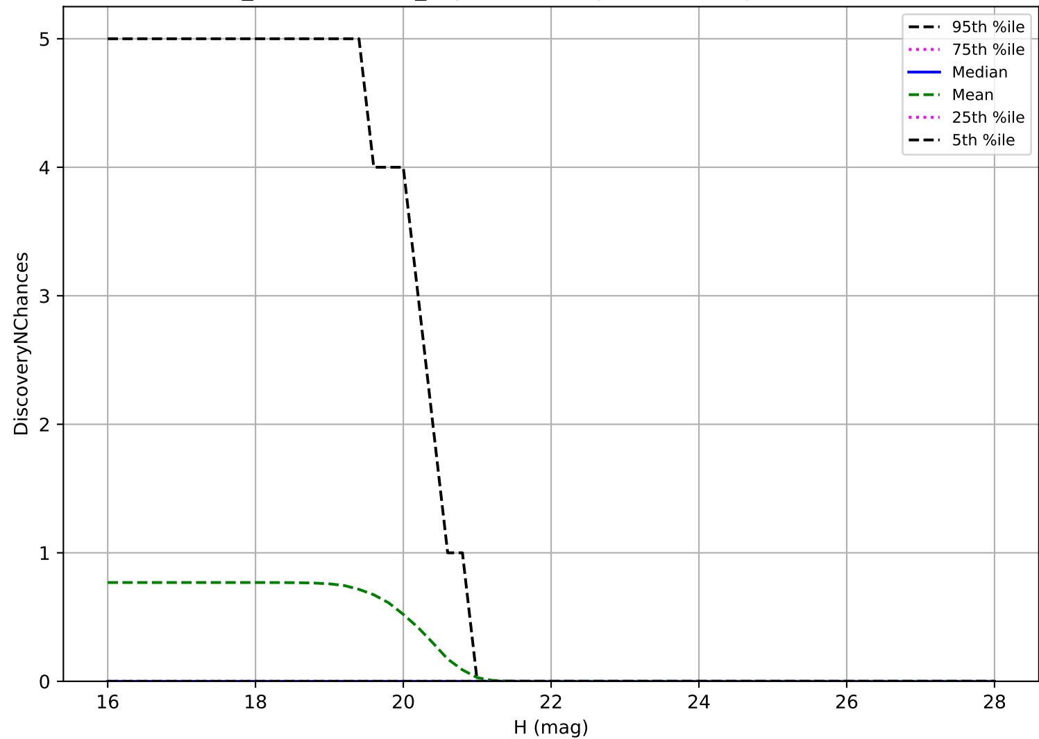
weather_cloudso30v3.4_10yrs: Vatira 3 pairs in 15 nights detection loss
