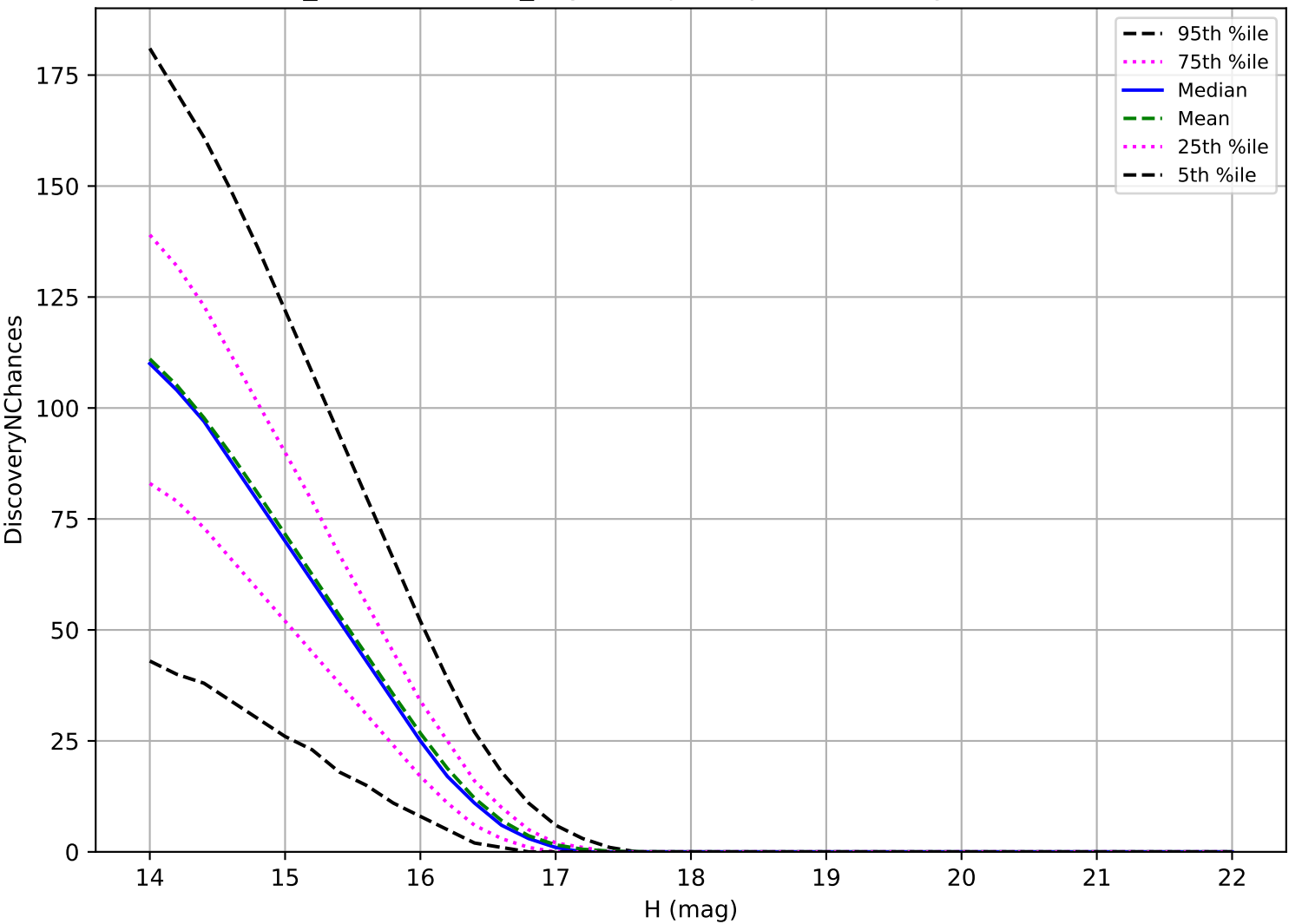
weather_cloudso30v3.4_10yrs: Trojan 3 pairs in 15 nights detection loss
