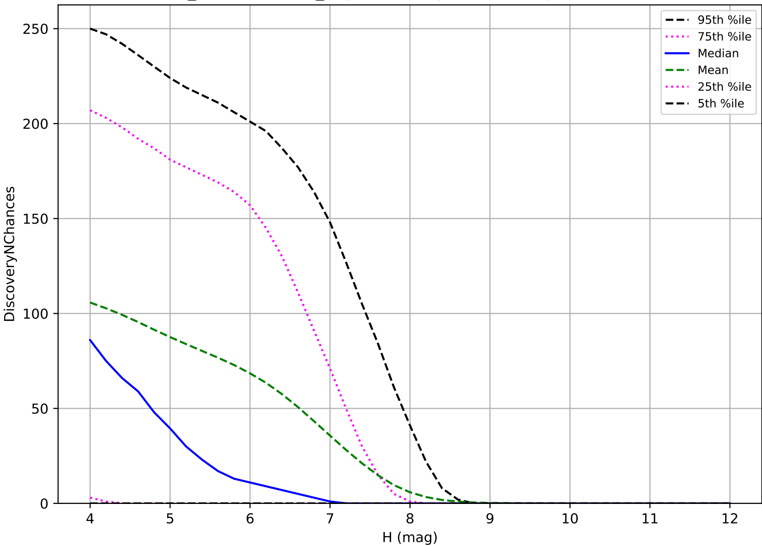
weather_cloudso30v3.4_10yrs: TNO 3 pairs in 15 nights detection loss
