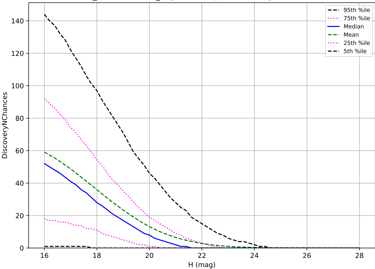
weather_cloudso30v3.4_10yrs: PHA 3 pairs in 15 nights detection loss
