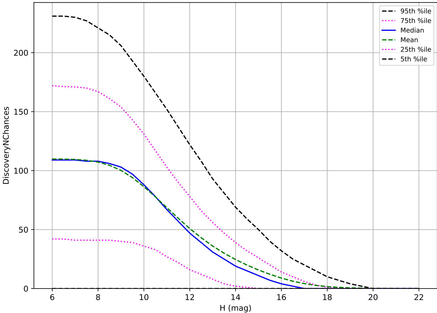
weather_cloudso30v3.4_10yrs: OCC_r5 3 pairs in 15 nights detection loss
