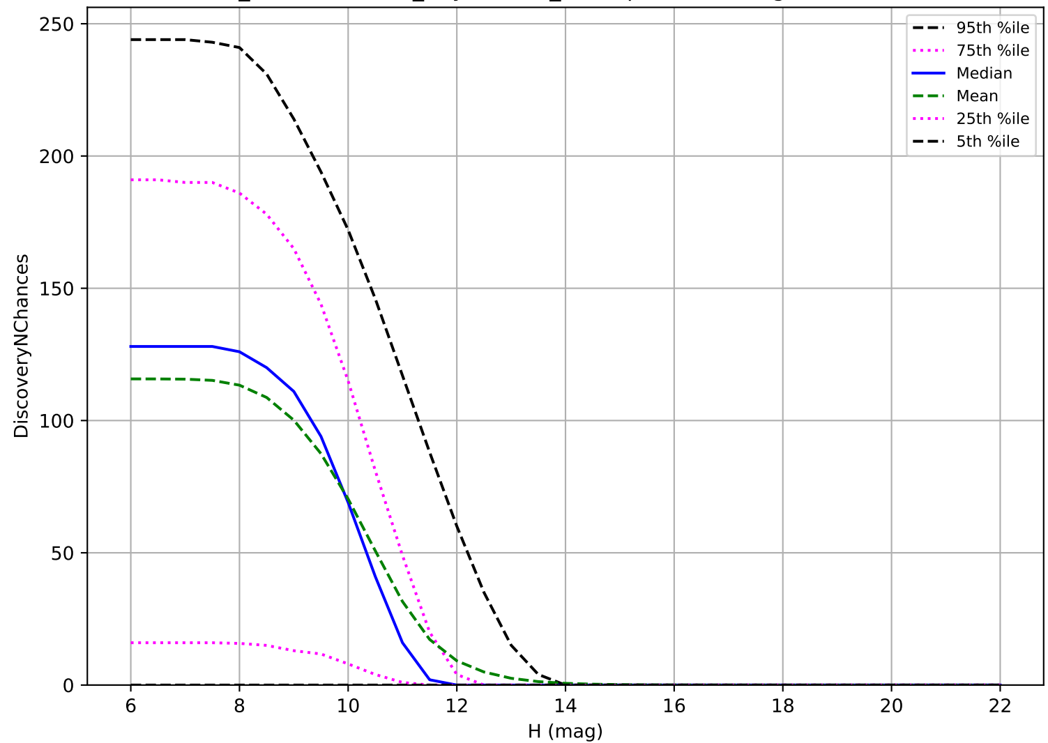
weather_cloudso30v3.4_10yrs: OCC_r20 3 pairs in 15 nights detection loss
