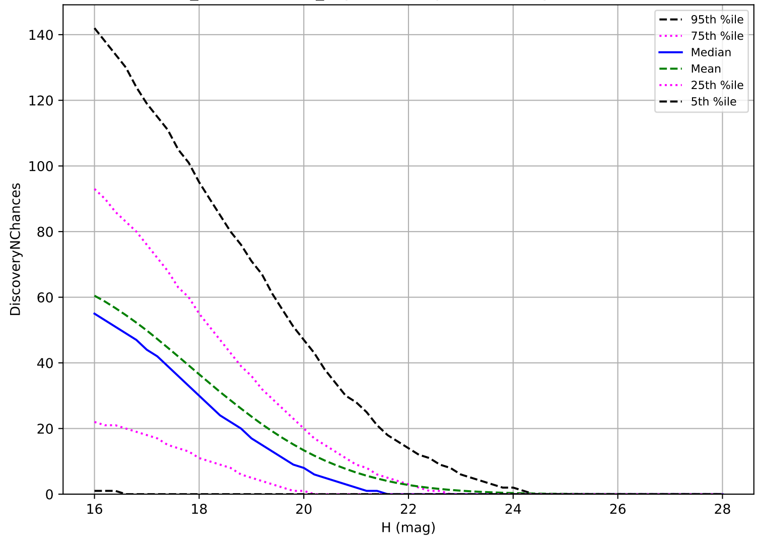
weather_cloudso30v3.4_10yrs: NEO 3 pairs in 15 nights detection loss
