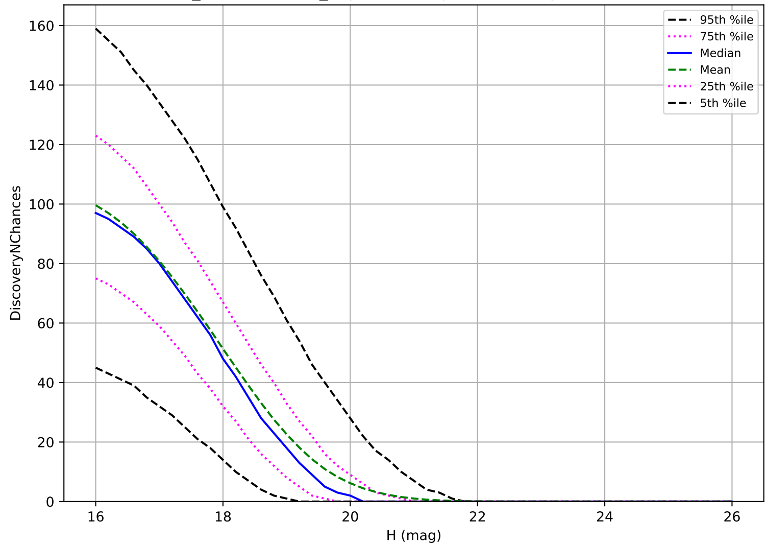
weather_cloudso30v3.4_10yrs: MBA 3 pairs in 15 nights detection loss
