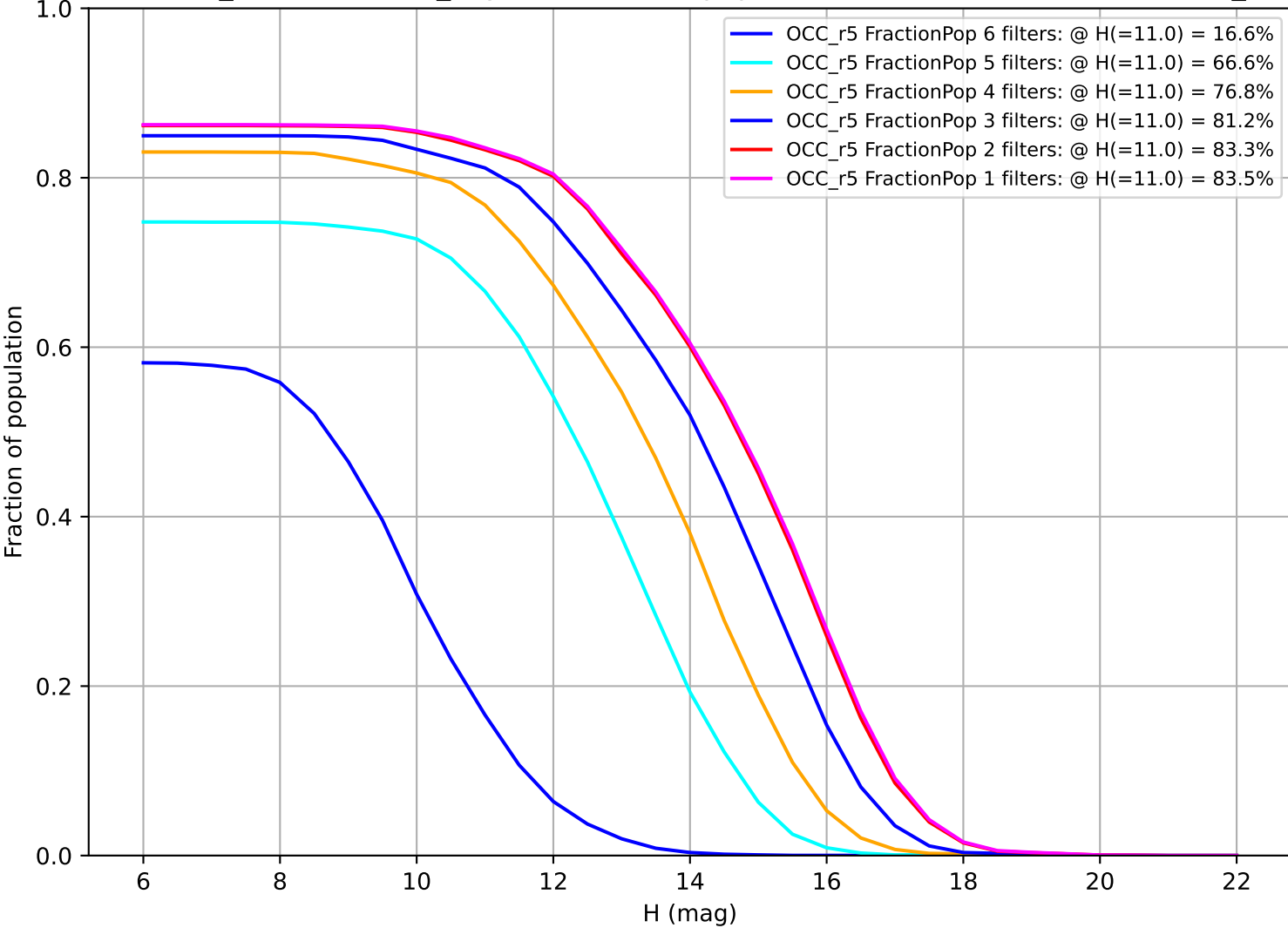
weather_cloudso30v3.4_10yrs: Fraction of population with colors in X filters OCC_r5
