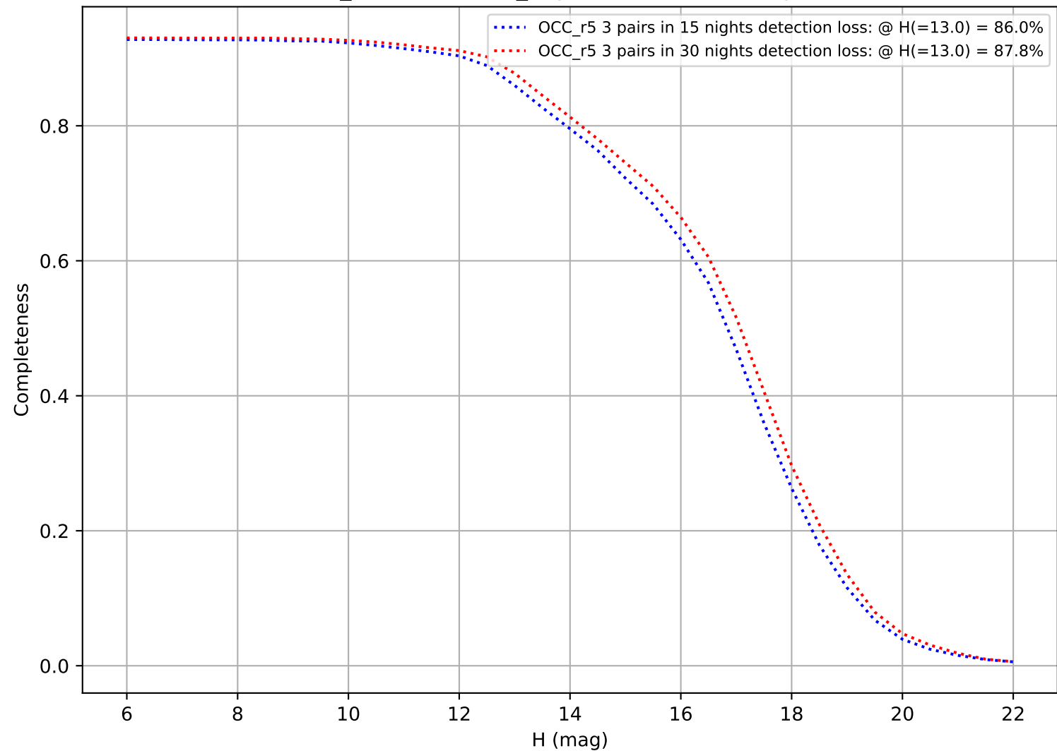
weather_cloudso30v3.4_10yrs: DifferentialCompleteness
