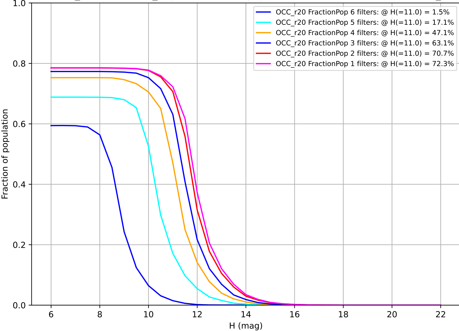
weather_cloudso30v3.4_10yrs: Fraction of population with colors in X filters OCC_r20
