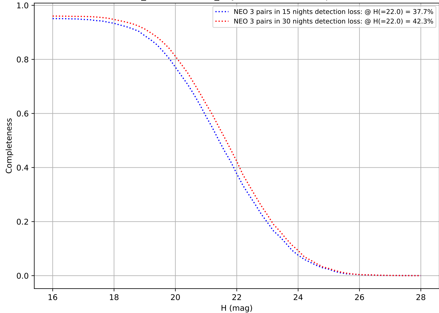
weather_cloudso30v3.4_10yrs: DifferentialCompleteness
