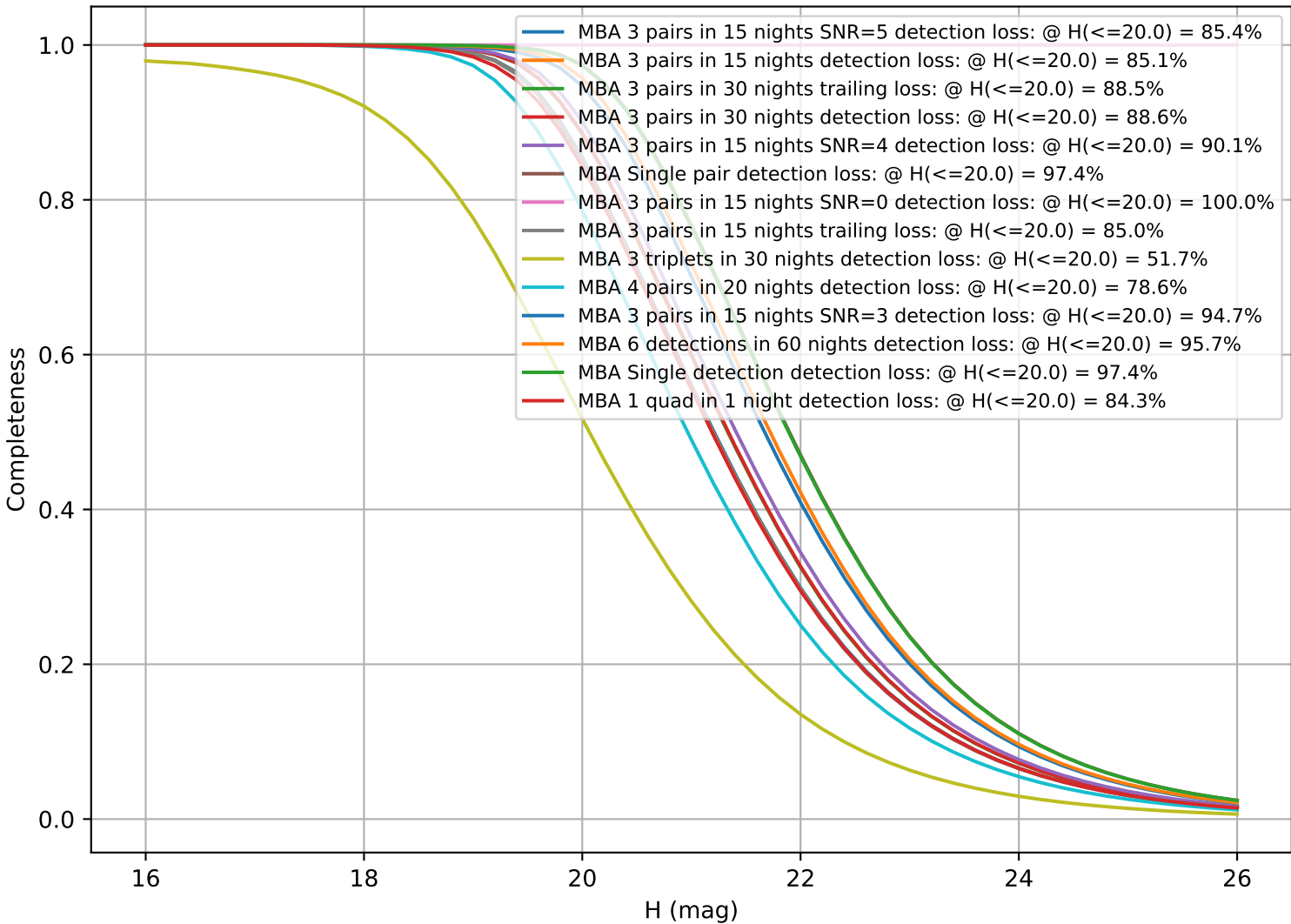
weather_cloudso30v3.4_10yrs: CumulativeCompleteness
