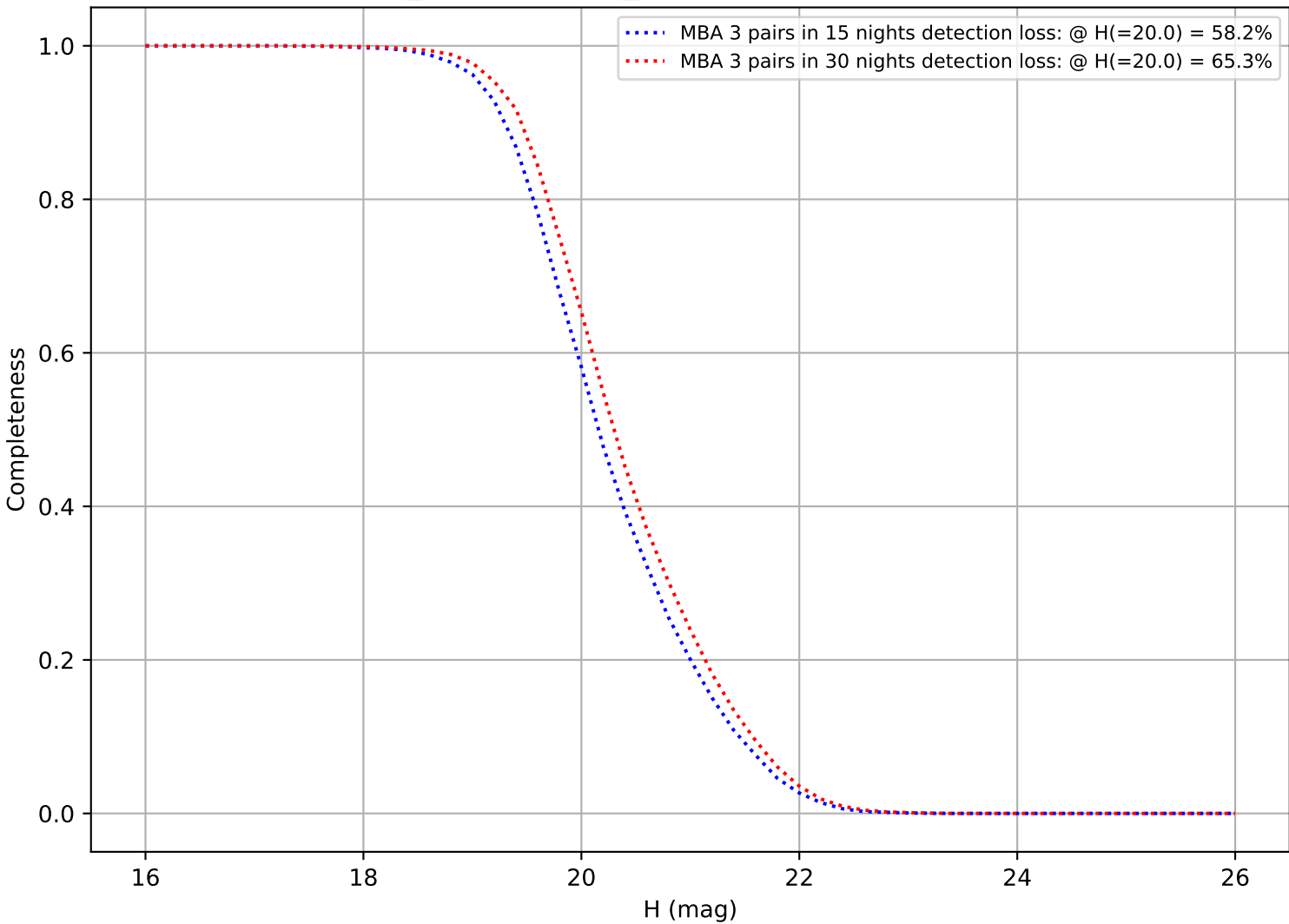
weather_cloudso30v3.4_10yrs: DifferentialCompleteness
